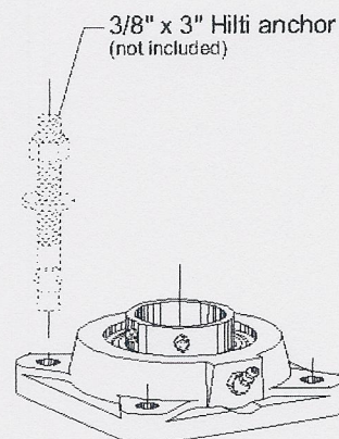
C9371 Grand bottom center pivot bearing
