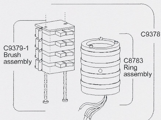
Grand revolver collector and brushes
