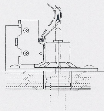
C9419 Lock indicator assembly
