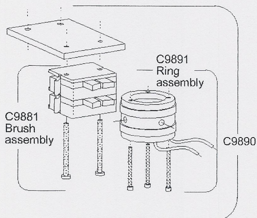
Standard revolver collector and brushes
