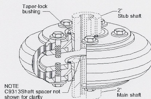
C9373-1 Coupling assembly
